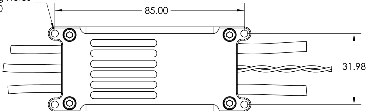
BOTTOM VIEW
